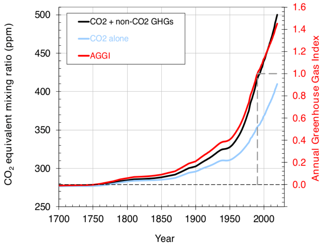
Figure 7.3. NOAA Annual Greenhouse Gas Index (updated Spring 2020). 106
